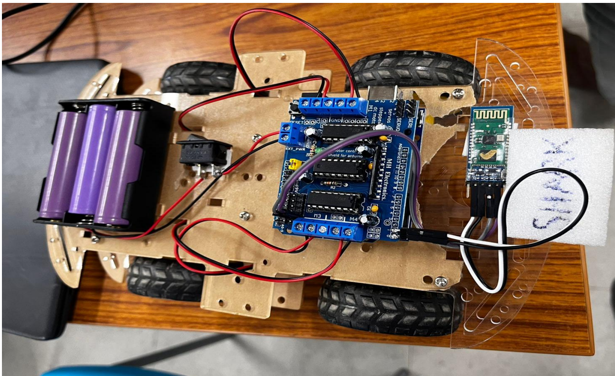
Hands on Training on Automatic Path tracing robot
